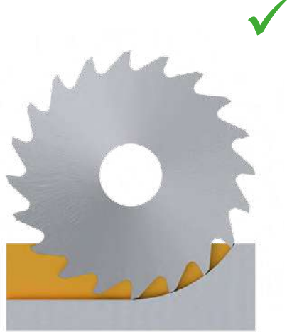
3 - 4 material teeth = stable machining
